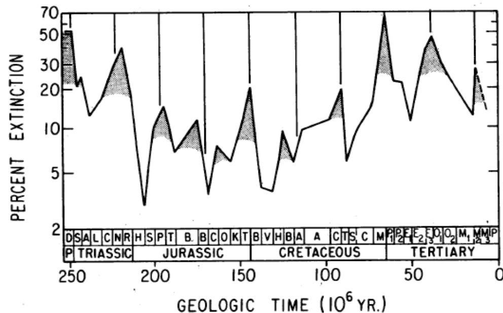
FIG. 1. Extinction record for the past 250 ma. Letter codes (bottom) identify stratigraphic stages. The best-fit 26-ma cycle is shown along the top. The relative heights of extinction peaks should not be taken as literal expressions of extinction intensity because the absence of extant taxa exaggerates the heights of younger peaks.
